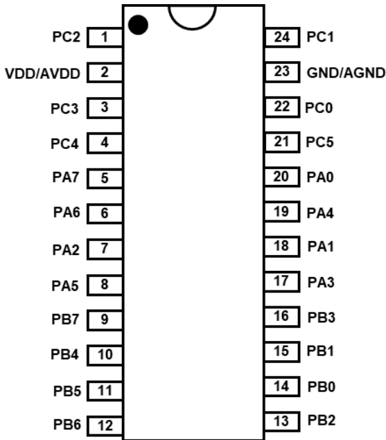
PGS134-S24: SOP24 (300mil)
