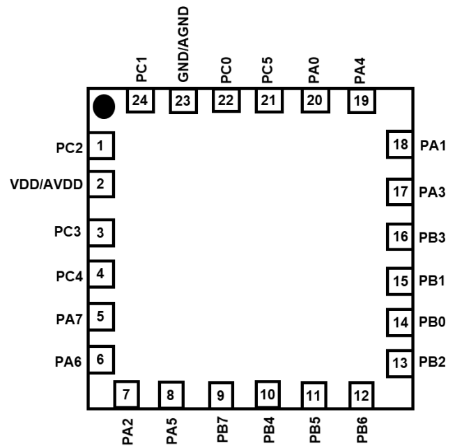
PGS134-2J24: QFN4*4-24P (0.5pitch)
